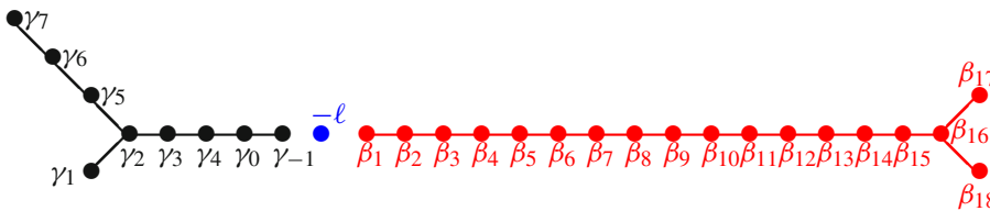
Reduced Dynkin diagram of D_{25}^{(2)} = E_7^{(1)} \diamond L \diamond D_{18}
