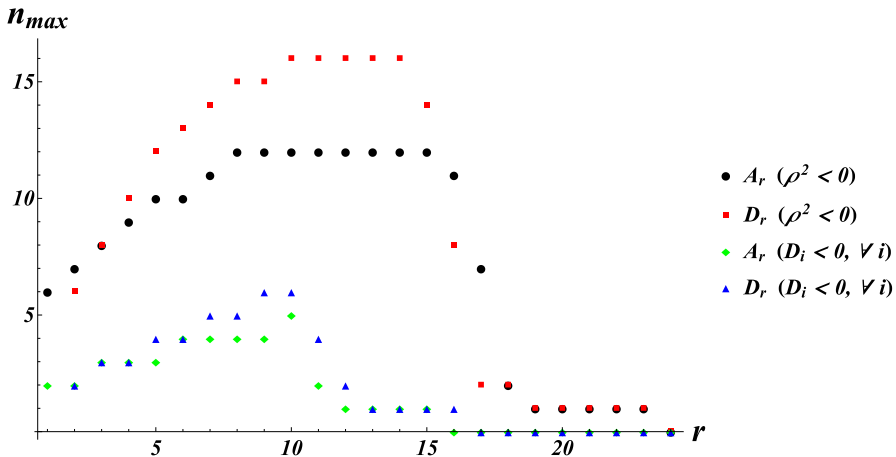
Fig. 1 Maximum values of n for \mathfrak{g}_{-n} with rank r to possess a SO(1, 2) -principal subalgebra from the necessary condition \rho^2 < 0 versus the necessary and sufficient condition D_i < 0, \forall i
