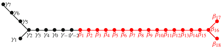
E_7^{(2)} \diamond D_{18} -Dynkin diagram on the root lattice for E_7^{(0)} \oplus \Pi^{1,1} \oplus \Pi^{1,1} \oplus D_{18}
