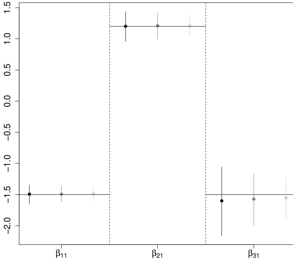
Figure 2: Linear coefficient estimates obtained by applying gjr to bivariate survival data with high censoring rates. Further details are given in the caption of Figure 1.
