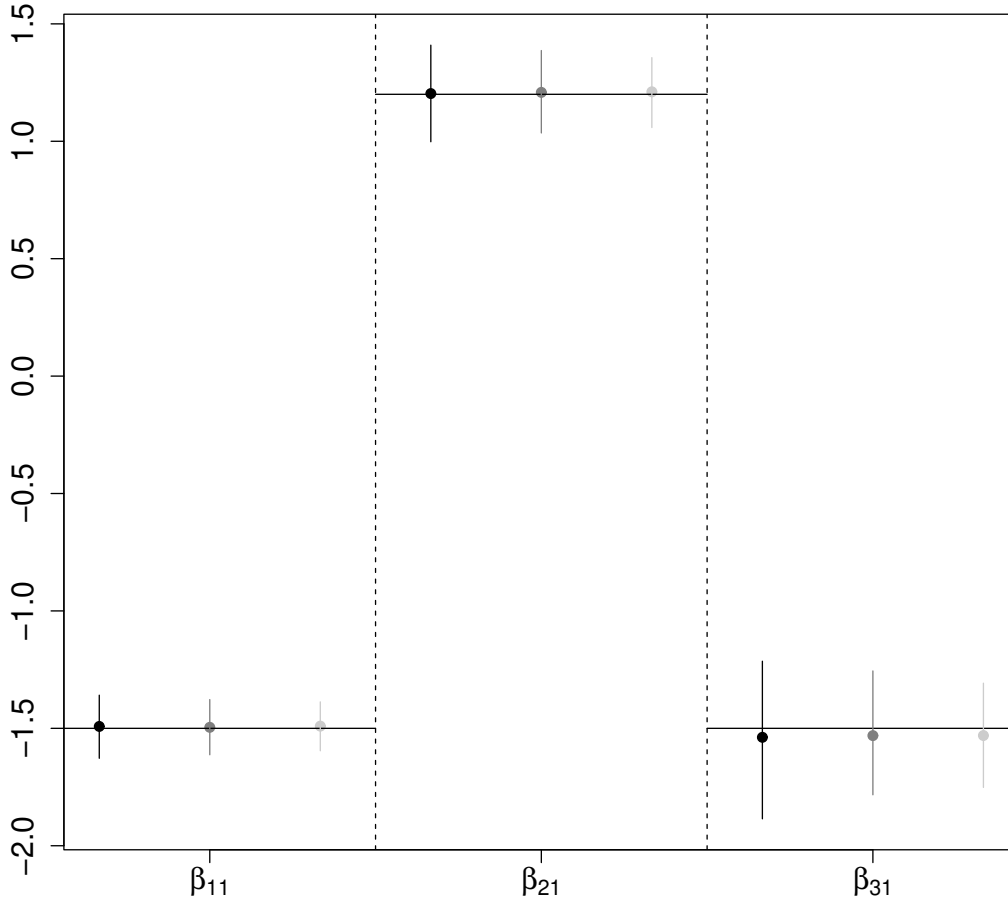
Figure 1: Linear coefficient estimates obtained by applying gjr to bivariate survival data with mild censoring rates. Circles indicate mean estimates, whereas vertical bars represent estimate ranges (5%-95% quantiles). True values are denoted with black solid lines. Black circles refer to the results obtained for n = 1000 , whereas those in dark grey and light grey are for n = 1500 and n = 2000 .
