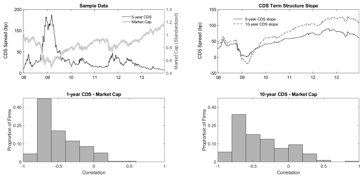
Figure 1. The Data: The figure summarizes daily data on market capitalization and CDS spreads between December 20, 2007, and December 19, 2013, for 164 firms. Data are obtained from Thomson Reuters. The top-left panel shows the average 5-year CDS spread (black line) and the standardized value of the market capitalization (gray line) across firms. CDS spreads are expressed in basis points. We compute the standardized value of the market capitalization for each firm as the ratio between the daily market capitalization and the value of the market capitalization on the first day of the time series, at the firm-level. The top-right panel shows the average 5-year (solid black line) and 10-year (dotted black line) CDS slopes across firms. We compute the daily 5(10)-year CDS slope as the difference between the daily 5(10)-year CDS spread and the 1-year CDS spread, at the firm-level. The bottom-left (right) panel shows the distribution of the firm-specific correlations between the 1(10)-year CDS spread and market capitalization.
