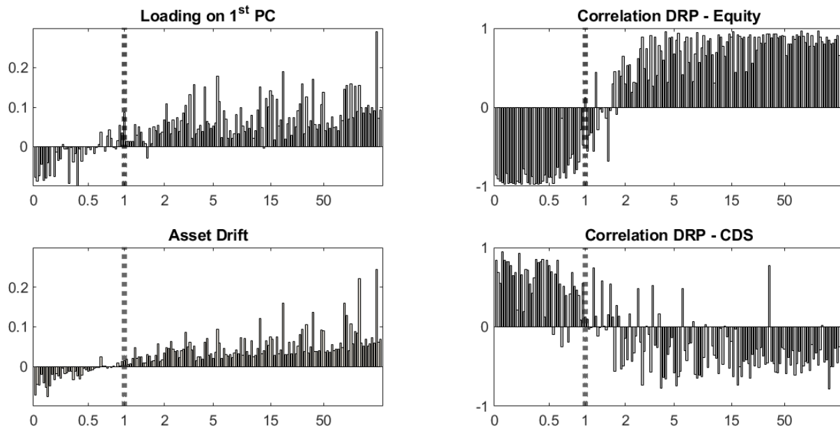
Figure 8. DRP Ranking: The figure shows the firm-specific loadings in the first PC obtained from PCA on the variance-covariance matrix of the implied market value of assets (top-left panel), correlations between daily default risk premium (DRP) and market capitalization over the sample time series (top-right panel), asset drifts \mu_V obtained from \mu_V = -(\mu_L - 0.5\sigma_L^2) using the estimated firm-specific \mu_L and \sigma_L (bottom-left panel), and correlations between daily DRP and 5-year CDS spread over the sample time series (bottom-right panel). In the x -axis, we report the firm-specific average 5-year DRP over time. The firms are ranked in ascending order according to their DRP.
