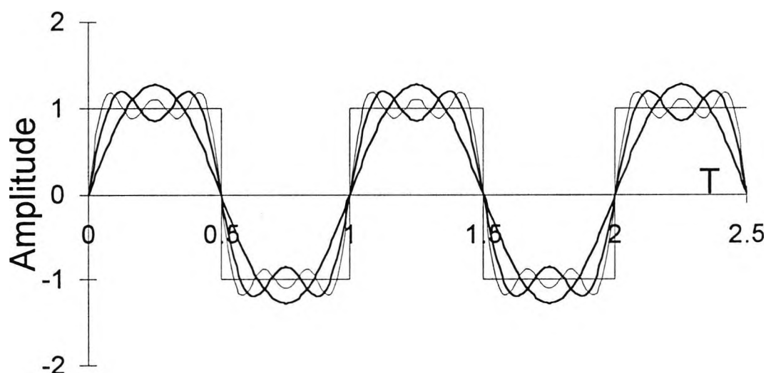
Figure 2-1. The cumulative sum of the first three terms of a truncated Fourier series of a square wave, and the square wave which they are summing to approximate.
