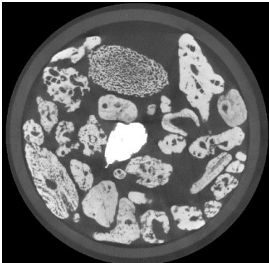
Figure 1. X-ray microtomography scan of São Tomé sand in a 30 mm diameter tube.
