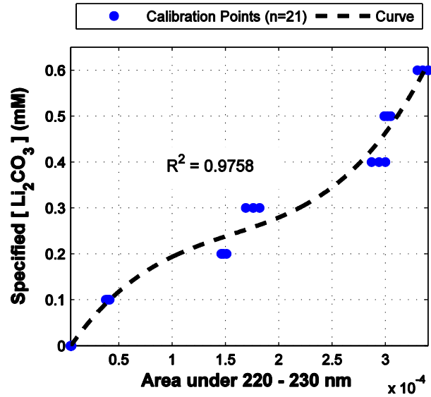
Figure 3: Calibration curve for Li 2 CO 3 in pure water.
