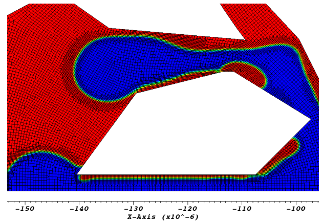
Figure 7: Snapshot for oil film capturing and water snap off using adaptive mesh. Blue represents water volume fraction and red oil.
