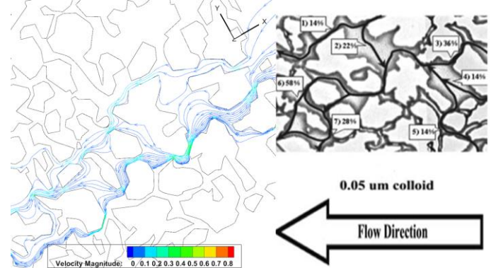
Figure 5: (a) Stream lines distribution with velocity vectors. Higher velocities are calculated at the upper part of the grain (b) Experimental results from Sirivithayapakorn et. al. (21) showing massless particle trajectory (thick black line)
