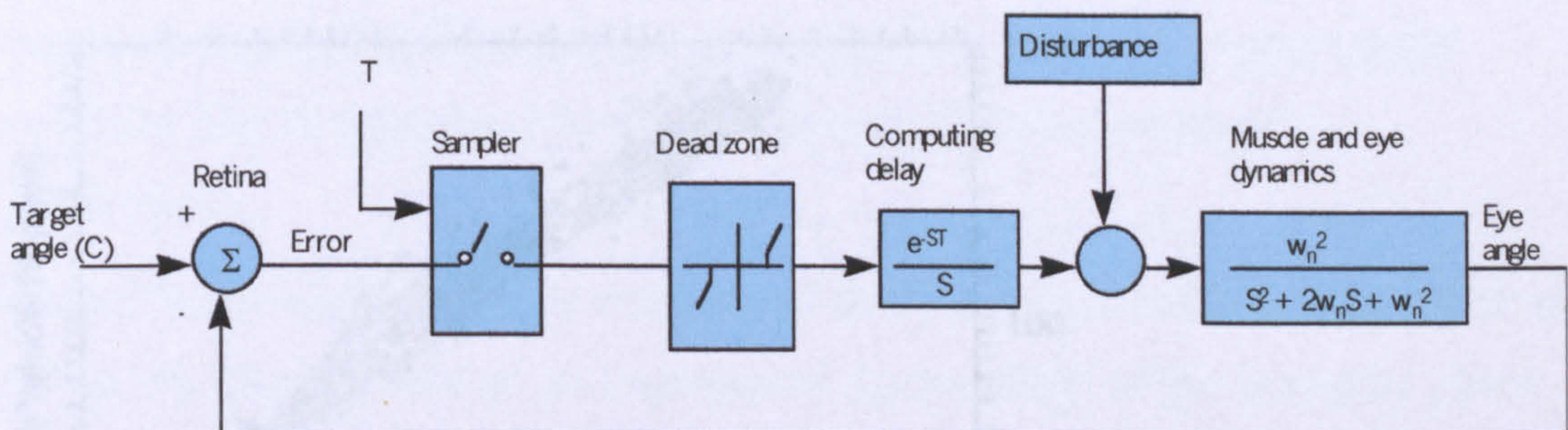
Figure 1.9. Sampled-data saccadic control model (from Young LR, 1981).
