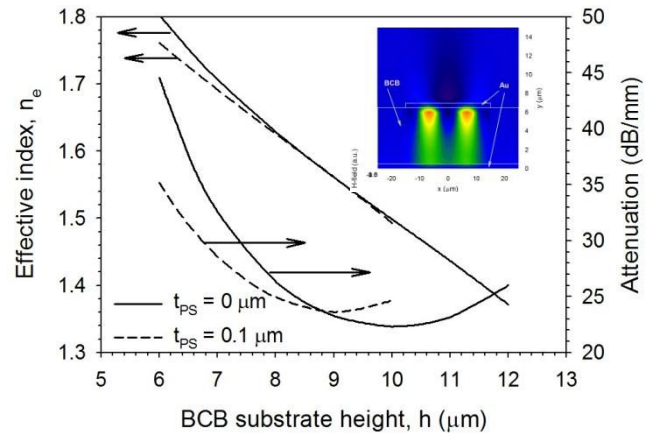
Figure 12 Variation of the effective index and attenuation with BCB substrate height of the microstrip line. (mode shown as inset)
