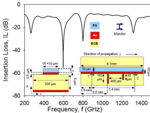
Figure 11 Insertion Loss with frequency for the microstrip filter
