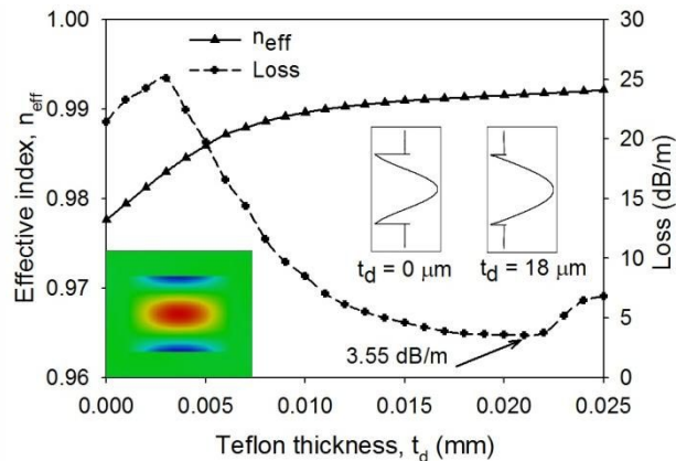
Figure 6. Effective index and loss with Teflon thickness for the H_{10}^x mode.
