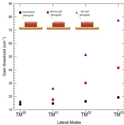
Figure 9. Gain Threshold of the lower order modes for different waveguides
