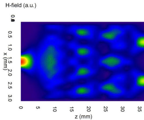
Figure 10 FDTD Simulation of the MMI 3dB coupler
