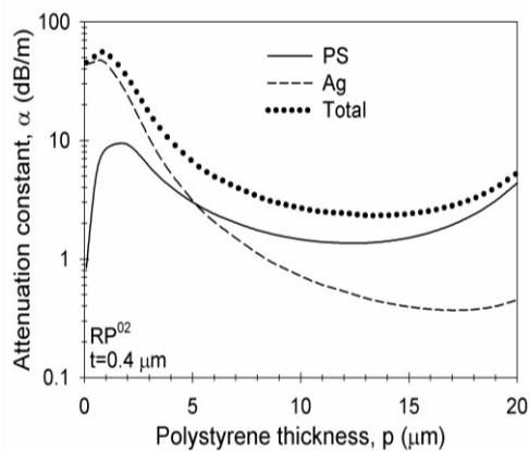
Figure 5. Attenuation constant with the polystyrene thickness, p , for t=0.4\mu\text{m} .
