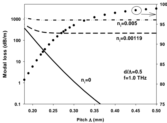
Figure 3. Material and leakage losses of PCF.
