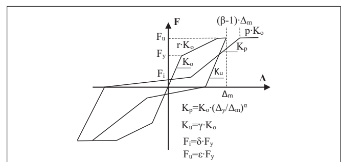
FIGURE 4 | Wayne-Stewart hysteretic model. Assumed hysteretic parameters for wood-frame buildings: \alpha = 0.38 , \beta = 1.09 , \gamma = 1.45 , \delta = 0.25 , \epsilon = 1.5 , and \rho = 0 .
