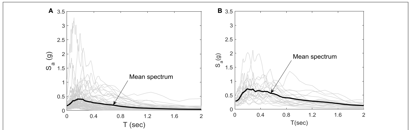
FIGURE 3 | Unscaled acceleration response spectra of ground motion records representative of (A) low to moderate seismicity records; (B) high-seismicity records.
