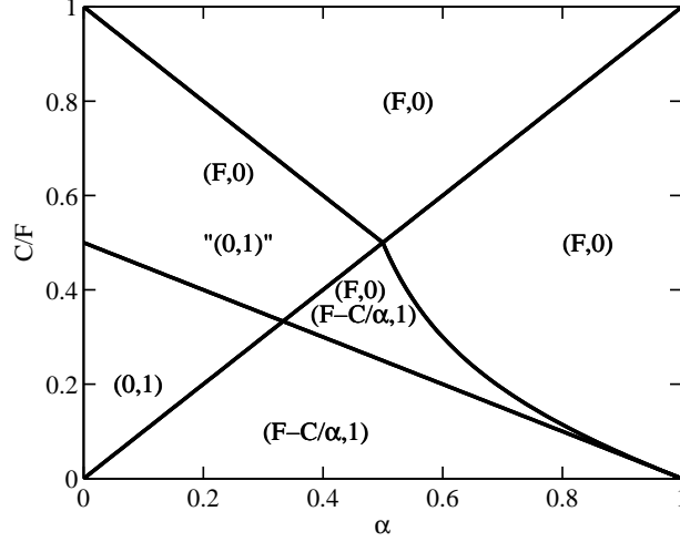
Figure 2: ESSs of the game for the asymmetric information case, where all terms are as defined in Table 1. The label “(0, 1)” denotes a region where there is an ESS of (0, 1) for the case of mistakes of the first kind (Finder plays Hawk for small values of a ). The label (0, 1) denotes a region where there is an ESS of (0, 1) for either kind of mistakes.
