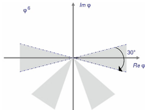
FIG. 2 (color online). Stokes' wedges (shaded regions) of angular opening 30^\circ in which the integration contour C for the integral \int_C d\phi \exp(-\phi^6) may terminate. The integral has two possible real values, one for which the contour connects the pair of wedges centered about the real axis and the other for which the contour connects the lower pair of wedges.
