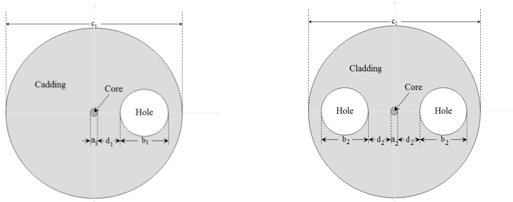
Figure 4.1 (a) One-hole high-birefringence fibre that has a hole diameter of 30\ \mu\text{m} and the distance between the right edge of the core to the left edge of the hole d_1 is 9\ \mu\text{m} . (b) Two-hole high-birefringence fibre that has two holes with the same diameter of 27\ \mu\text{m} and the distance between the right edge of the core to the left edge of the hole on the right d_2 is 14\ \mu\text{m} .
