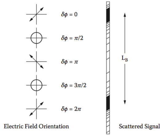
Figure 3.8 Visual determination of the beat length, L_B , with the optical phase difference between the two orthogonal polarization states[233].
