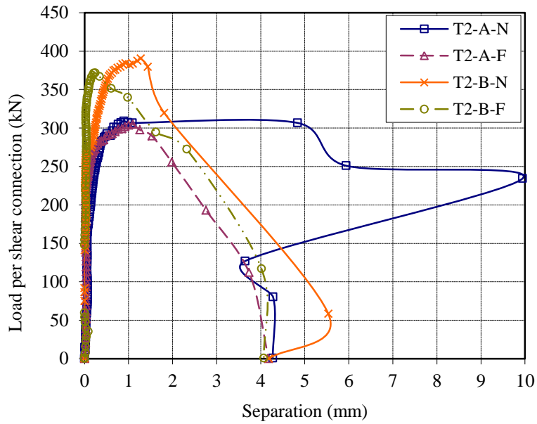
Fig. 13. Load-slip and load-separation curves of the tie-bar ( \text{\O}12\text{mm} ) shear connection in test group T2
