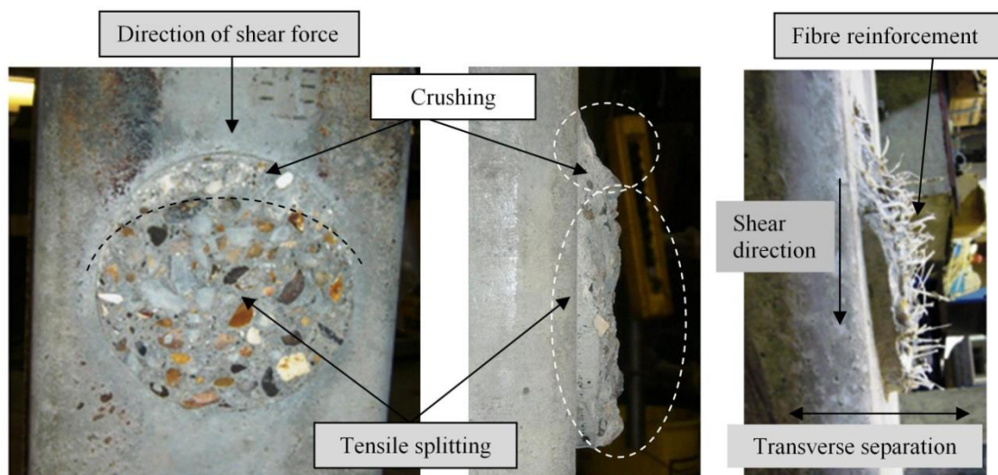
Fig. 21. Failure profiles of the concrete-infill-only shear connection
