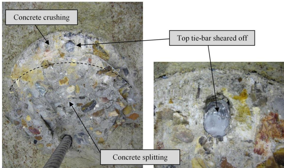
Fig. 22. Failure profiles of the tie-bar ( \text{Ø}12\text{mm} ) shear connection
