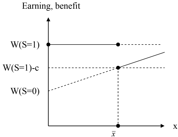
Figure 1: Earnings and regional ethnic concentration ( x )
