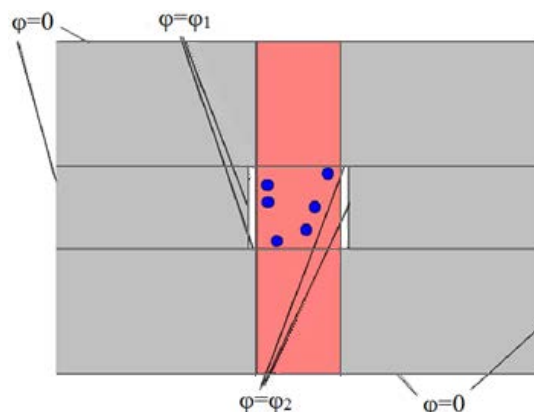
Figure 2. 2D finite element model showing boundary conditions.
