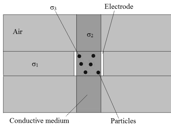
Figure 1. Basic 2D finite element (FE) model of particles in a conductive medium.
