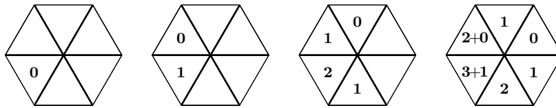
Fig. 10: The first four steps of running Soergel’s cancellation-free algorithm along \omega^\gamma . We have recorded the powers of the polynomials only (for example, 2 + 0 should be read as t^2 + t^0 ).
