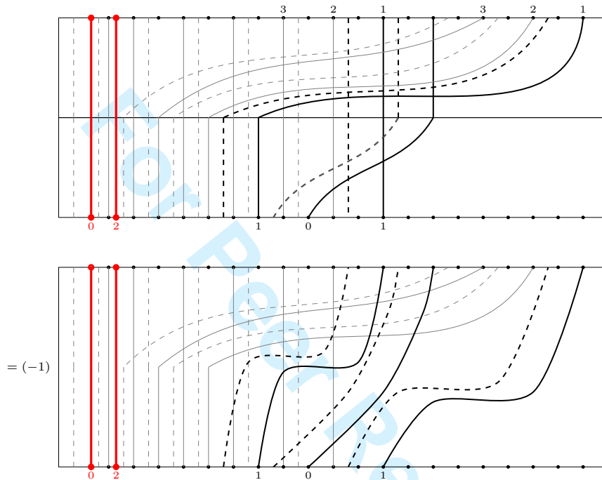
Fig. 26: The top diagram is obtained by concatenation of the diagram 1_1^{2'} above 1_0^1 . The lower diagram is obtained by applying relation (2.10) to the product 1_1^{2'} \circ 1_0^1 . We move the ghost 0 strand through the crossing pair of black strands of residue 1 (we do not record the diagram which is zero modulo more dominant terms).
