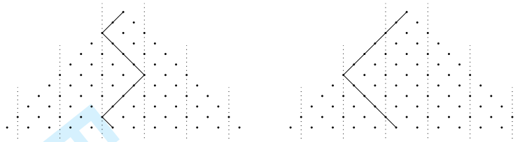
Fig. 8: Two paths \omega'', \omega''' \in \text{Path}((6, 5), \omega^{(0,11)}) .
