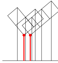
Fig. 12: The diagram and loading of the bipartition ((2, 1), (1^3)) for \ell = 2, g = 1, \theta = (0, 0.5) .
