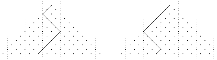
Fig. 7: Two paths \omega, \omega' \in \text{Path}((4, 7), \omega^{(0,11)}) .
