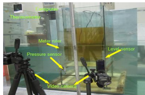
Fig.3 Experimental equipments
