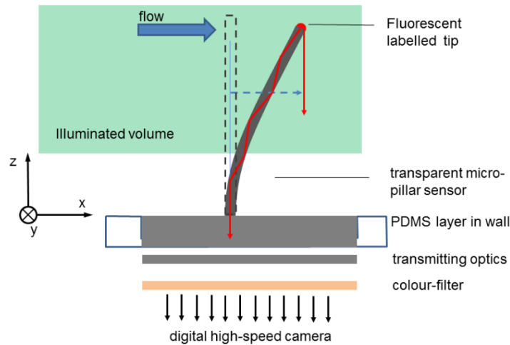
Fig. 1. Set-up of the subcutaneous recording of the pillar tip deflection using fluorescently labelled tips of the transparent pillars and their wave-guidance properties. The blue arrow indicates the relevant measure of tip displacement Q relative to the no-flow situation that is captured by the imaging system below the wall.
