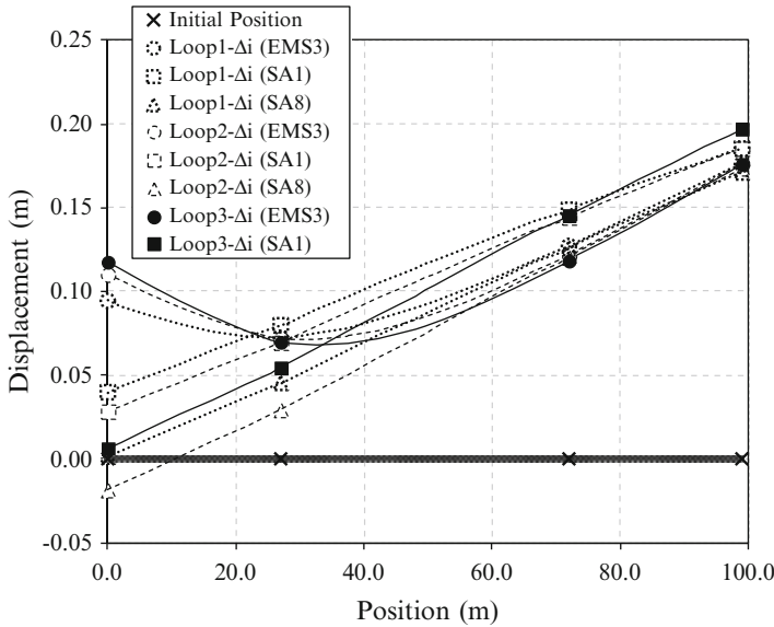
Fig. 7.6 Target-displacement profiles \Delta_i (EMS), structural analysis displacement profiles (SA1) based on the secant stiffnesses of EMS and revised structural analysis displacement profiles (SA) that converge to the target-displacement of the critical member (i.e. Abt2) and Col2, derived iteratively from the DDBD methodology
