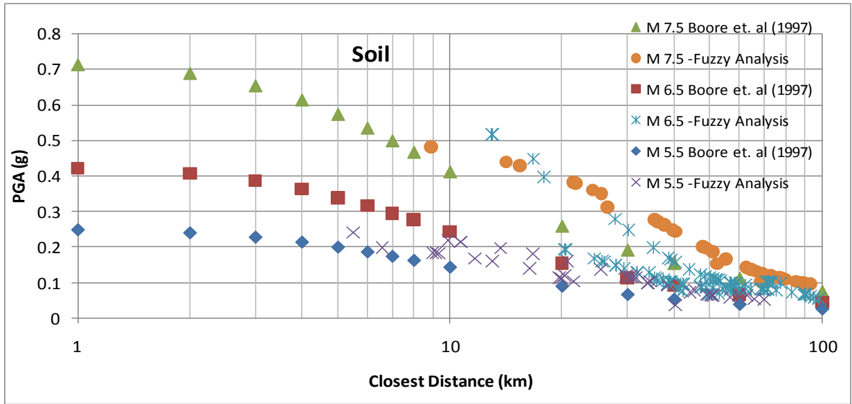
Figure 10. Curves of peak acceleration versus distance for magnitude 5.5, 6.5 and 7.5 earthquakes at soil sites.
