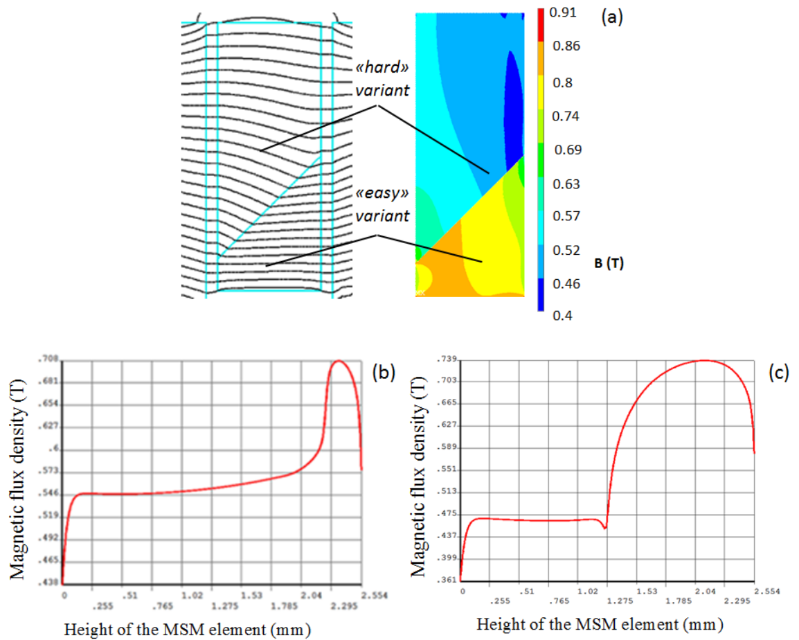
Figure 4.3-9. (a) Magnetic field lines and flux density distribution in the MSM element with a single twin boundary, and x- component of magnetic flux density calculated in the air gap near (b) left and (c) right surface of the MSM element
