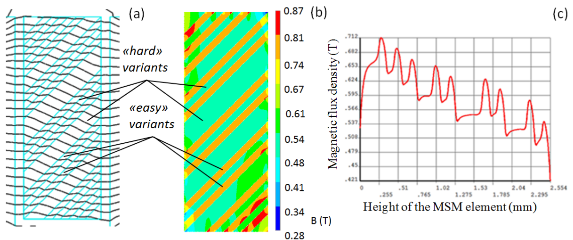
Figure 4.3-3. (a) Magnetic field lines and (b) flux density distribution in the MSM element with fine twins, (c) x- component of magnetic flux density in the air gap near the left surface of the MSM element
