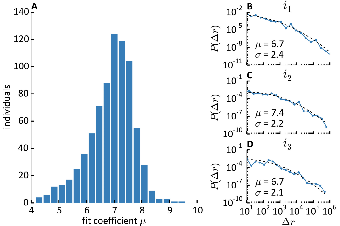
Fig 4. Distribution of individual displacements. A ) Frequency histogram of 96.2% of individuals for which the individual distribution of displacement is log-normal, according to the value of the log-normal fit coefficient \mu . B-C-D ) Examples of the distribution of displacements P(\Delta r) of three individuals i_1 (B), i_2 (C), i_3 (D) (dotted line), with the corresponding log-normal fit (dashed line). The value of the fit coefficients \mu and \sigma are reported in each subfigure.
