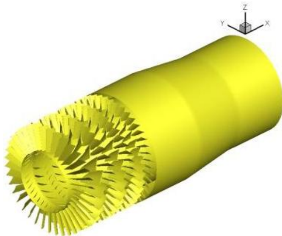
Fig. 2: Computational domain of the IDAC compressor for unsteady time-accurate simulation
