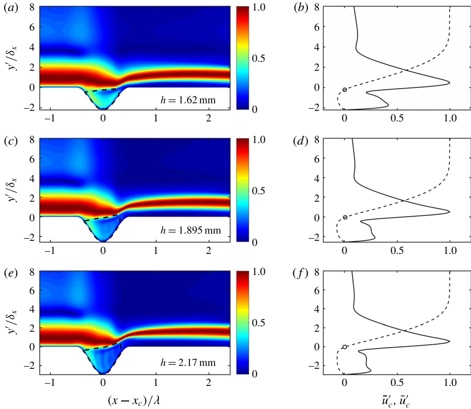
FIGURE 11. (Colour online) Comparisons of |\tilde{u}'(x', y', z')|/A'(x', z') contours (a,c,e) in the planes z' = 0 and corresponding TS mode profiles |\tilde{u}'_c| = |\tilde{u}'(x', y', z')|/A'(x', z') and |\tilde{v}'_c| = |\tilde{v}'(x', y', z')|/A'(x', z') (b,d,f) at x' = x'_c in the planes z' = 0 . The parameter \lambda = 40.5 mm. (a,b) h = 1.620 mm; (c,d) h = 1.895 mm; (e,f) h = 2.170 mm. In (a,c,e), the dashed lines indicate the interfaces of the regions enclosed by \Gamma = \{(x', y') : \tilde{u}'(x', y', z'=0) = 0\} and in (b,d,f), the solid lines indicate the profiles of |\tilde{u}'_c| and the dashed lines indicate the profiles of |\tilde{v}'_c| and o indicates the position where \tilde{u}'_c = 0 .
