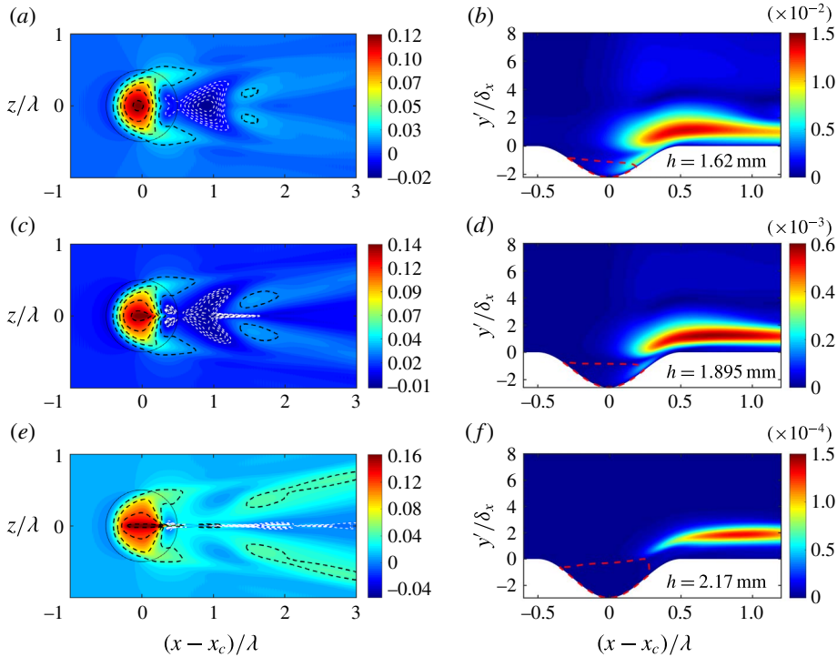
FIGURE 7. (Colour online) Comparisons of streamwise growth rate \alpha'_\varepsilon contours (a,c,e) and rescaled TS amplitude |\tilde{u}'(x', y', z')|/A'(x'_{neutral}, z') contours (b,d,f) where A'(x'_{neutral}, z') means amplitude of TS waves at the lower branch of the neutral stability curve. The parameter \lambda = 81 mm. (a,b) h = 1.620 mm; (c,d) h = 1.895 mm; (e,f) h = 2.170 mm. In (a,c,e), the black dashed lines indicate destabilisation of TS waves and the white dashed lines indicate stabilisation of TS waves ( -\alpha'_\varepsilon \leq 0 ). The solid circles are the curves of r = \lambda/2 . In (b,d,f), the red dashed lines indicate the interfaces of the regions enclosed by \Gamma = \{(x', y') : \tilde{u}'(x', y', z') = 0\} .
