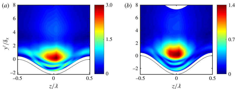
FIGURE 14. (Colour online) Experimental results of |\tilde{u}'(x', y', z')|/A'(x'_{neutral}, z') which correspond to the results given in figure 13 for the case h = 1.620 mm (a) and the case h = 2.170 mm (b). The parameter \lambda = 81 mm.
