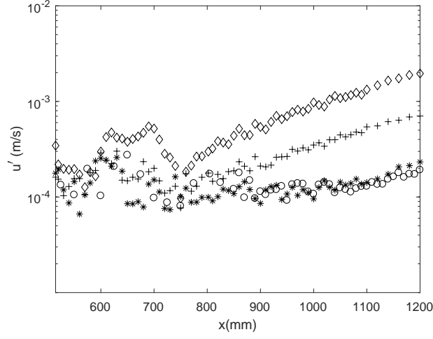
Figure 5: The amplitude of TS wave along the streamwise direction, for the unexcited case and the excited cases where the TS mode was extracted at f = 120Hz , f = 172Hz and the first harmonic mode ( 2f ) of the excitation at f = 86Hz , represented by '○', '*', '◇' and '+' and respectively.
