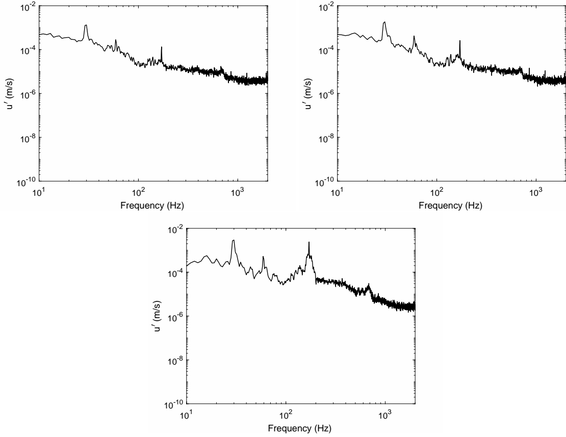
Figure 6: FFT of the fluctuating hot wire signal at a constant excitation frequency, f = 172Hz , but varying voltage input to the motors, top-left, V_{rms} = 2.0V , top-right, V_{rms} = 2.5V and bottom V_{rms} = 3.2V . The measurements were at x = 1200mm and y \approx 1.5mm .
