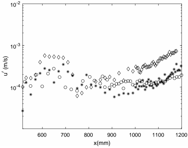
Figure 10: The amplitude of TS wave along the streamwise direction, for the unexcited case and the excited cases where the TS mode extracted f = 120Hz , f = 172Hz and the mode of the first harmonic ( 2f ) of the excitation at f = 86Hz , represented by 'o', '*', '+ and '◇'.
