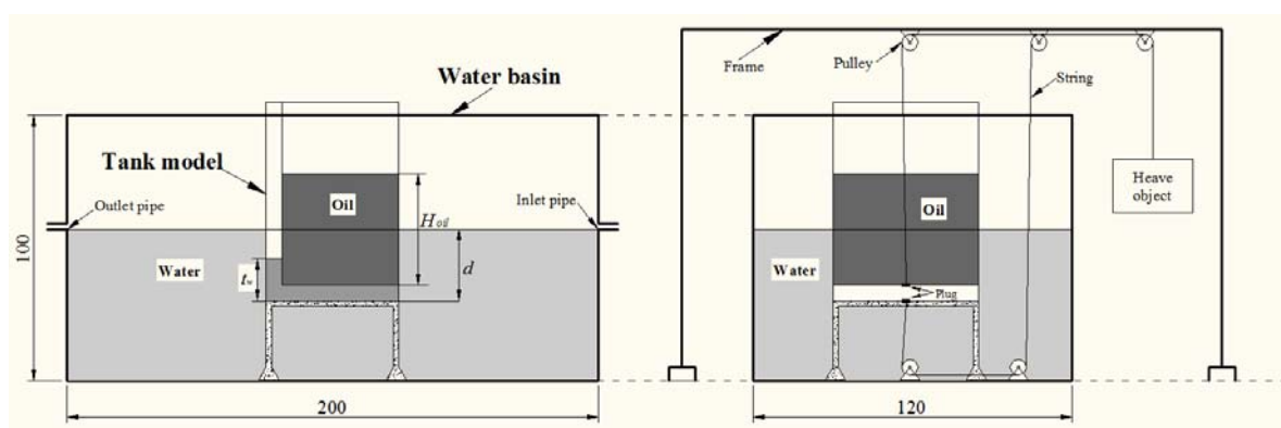
Figure 3.2 Sketch of the experiment configuration (unit: cm).
