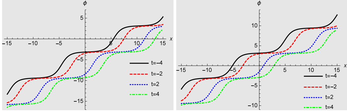
Figure 3: Sine-Gordon cnoidal kink solution \phi_{+,m,\beta}^{>(1)}(x,t) (panel a) and degenerate cnoidal kink solution \phi_{+,m,\beta}^{c>}(x,t) (panel b) for spectral parameter \beta = 0.9 and m = 0.3 at different times.
