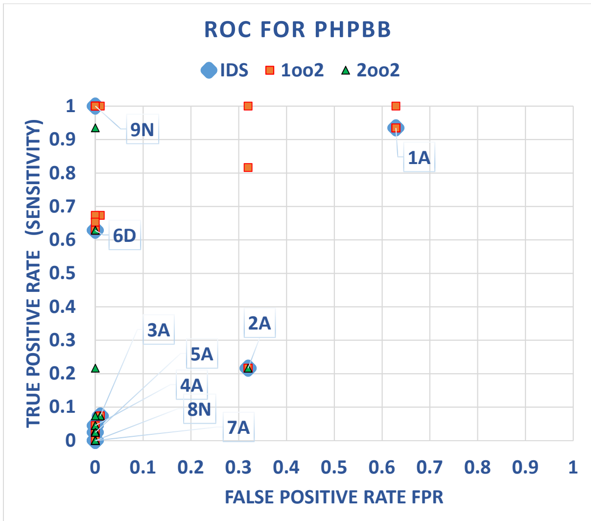
Figure 12 ROC PLOT SHOWING THE INDIVIDUAL IDSs, 1002 AND 2002 CONFIGURATIONS FOR PHPBB
