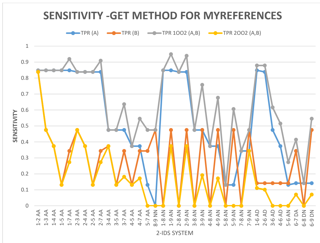
Figure 44 THE SENSITIVITY FOR A GIVEN SYSTEM A WHEN PAIRED WITH ANOTHER SYSTEM B FOR MYREFERENCES, THE CHART SHOWS THE INDIVIDUAL IDSs, 1002 AND 2002 CONFIGURATIONS WHEN ATTACKS WHERE READ (GET)
