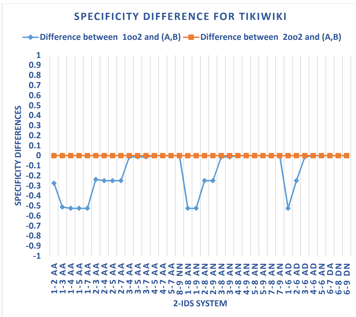
Figure 29 THE SPECIFICITY DIFFERENCE OF 1002 AND 2002 CONFIGURATIONS, COMAPRED WITH THE BEST SINGLE SYSTEM IN THE RESPECTIVE PAIR FOR TIKIWIKI
