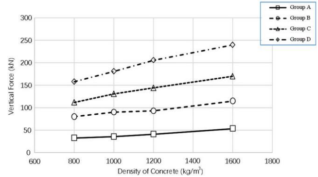
Fig. 5 Peak Force versus Foam Concrete Density
