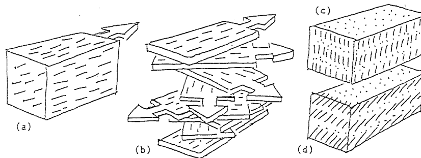
FIGURE 2.36 Liquid crystal mesophase structures: (a) Nematic, (b) Cholesteric, (c) Smectic A, (d) Smectic C.
