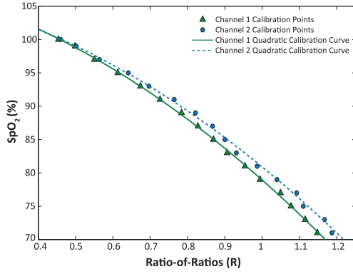
Fig. 12. Calculated R-values of the channel-1 (solid line) and channel-2 (dotted line) plotted against the set SpO_2 values.
