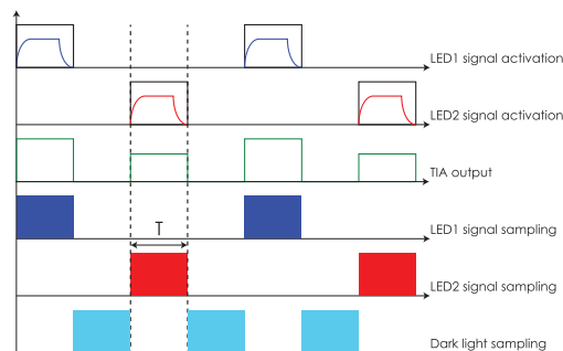
Fig. 4. PPG signal sampling at two different wavelengths using time windowing.
