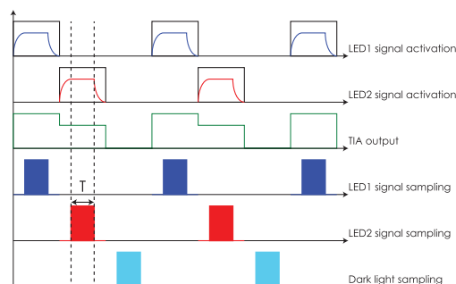
Fig. 5. Time windowing solution for avoiding switching noise, by sampling at the plateau of the LED on time.
