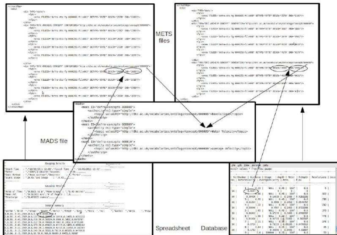
Figure 4 Encoding data component linkages with METS and MADS
