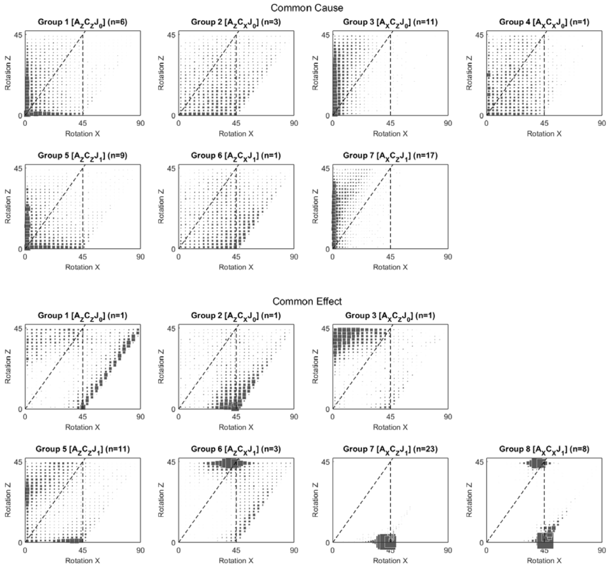
Fig. L1. Joint posterior probability density of the rotation parameters of the QPC model. The parameters are continuous but have been binned for this plot. The size of squares shows the value of the joint posterior probability density of the parameters within each cluster. Each cluster also shows the preferred projection orders for that cluster, and the number of participants for which this was the model cluster.
