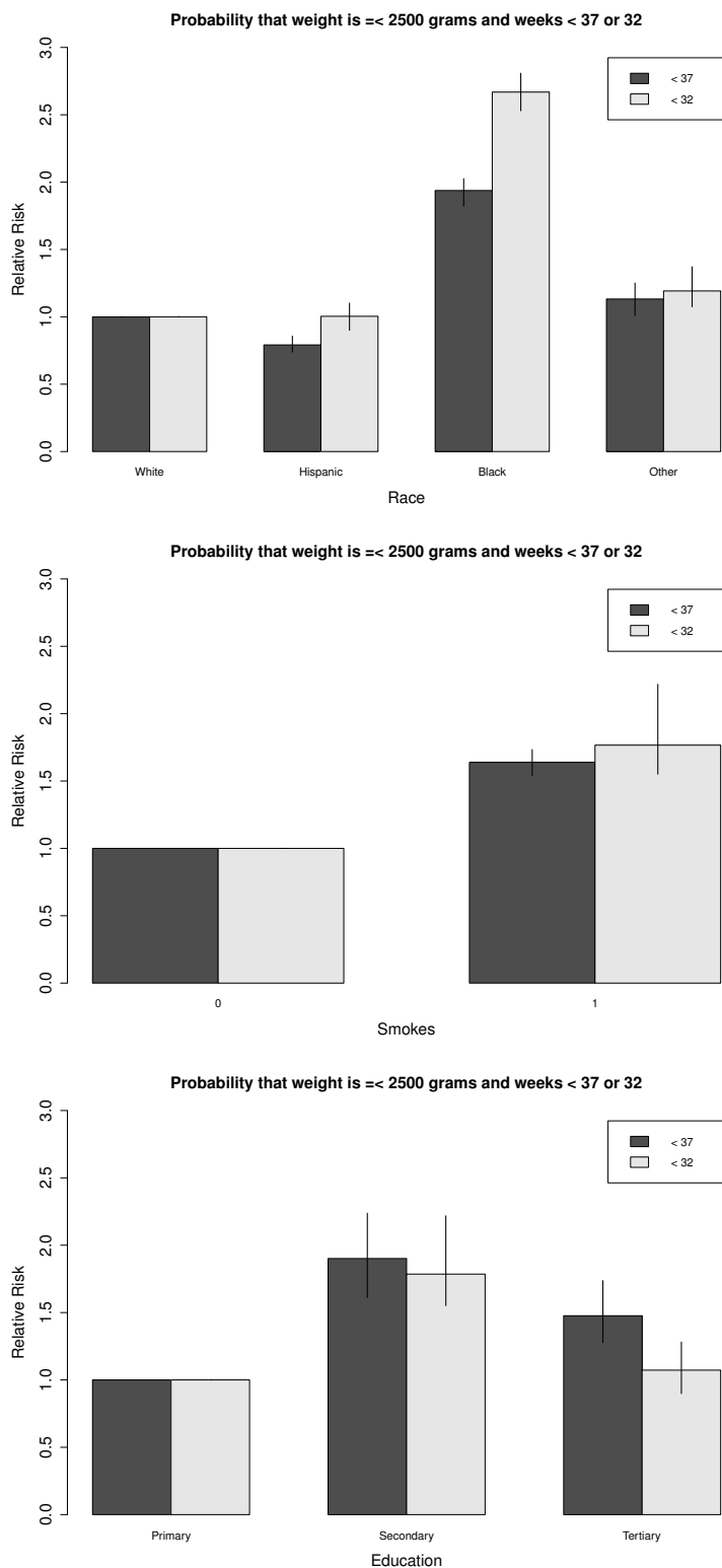
Figure 3: Joint probabilities for being low birth and being born before 37 weeks and 32 weeks by race, smoking behavior and education. The results are presented in terms of relative risk ratios where the baseline categories are white, non-smoker and primary, respectively. Variable age was set to its average, whereas the other factor variables were set to the respective categories with highest frequencies.
