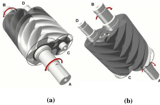
Fig. 1 Screw compressor rotors
