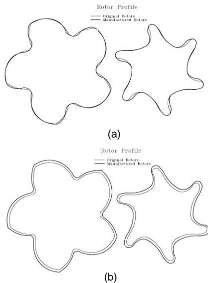
Fig. 13 (a) Effect of an error of 0.1^\circ in the tool-rotor shaft angle; (b) Effect of an error of 50\ \mu\text{m} in the tool-rotor centre distance
