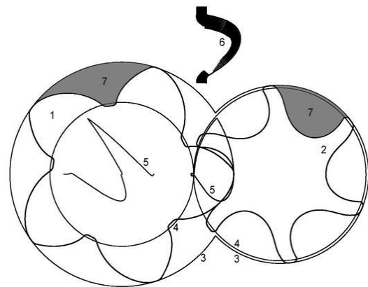
Fig. 2 Screw rotor profile
