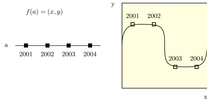
Fig. 5.2 Examples of 1-to-2 layout. In the figure, function f maps one variable to the two visual dimensions x and y . This case covers special cases such as the use of trigonometric functions.
