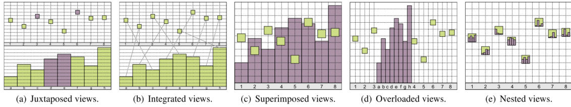
Fig. 2.6 Visual composition methods from Javed and Elmqvist (2012): (a) juxtaposition, (b) integration, (c) superimposition, (d) overloading and (e) nesting.
