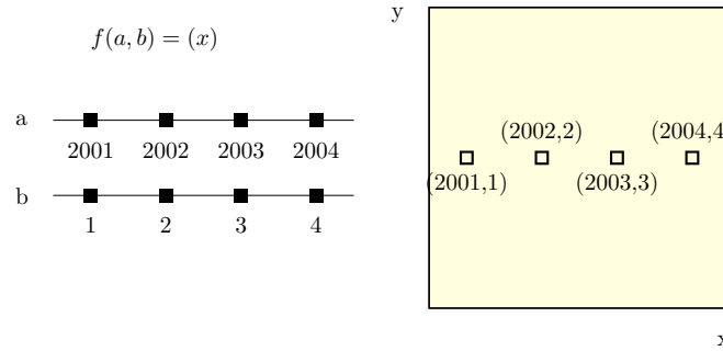
Fig. 5.3 Examples of n-to-1 layout. In the figure, function f maps two variables to a single visual dimension x ; in the example, y remains constant. This case covers dimensionality reductions where multiple attributes are used to derive a position.
