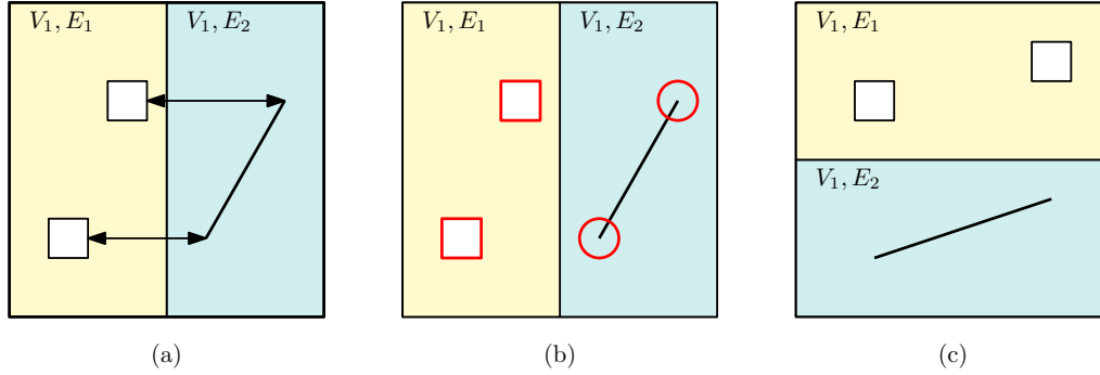
Fig. 4.7 Example of same level juxtaposition with different encoding: (a) shows the use of explicit linking connecting visual marks in each view; (b) represents the use of a shared encoding, a red outline, to identify marks in both views; (c) displays a variation of spatial arrangement
