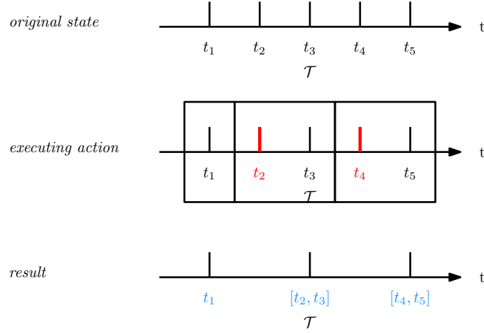
Fig. 6.8 Application of the Bin at Instants operator, with time points t_2 and t_4 passed as parameter. In executing action , the matched parameters are shown in red and the resulting segments enclosed. The lower part of the figure contains the resulting three time points, where two of them contain two instants.
