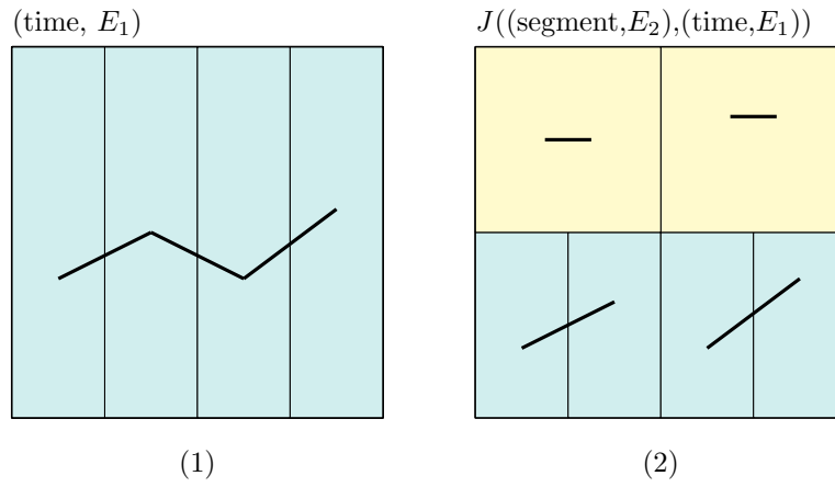
Fig. 7.5 Example of segmenting and juxtaposing between levels.
