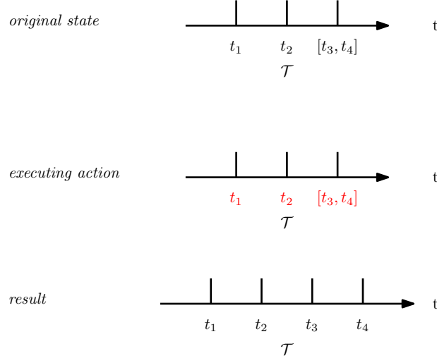
Fig. 6.11 Application of the Expand operator.
