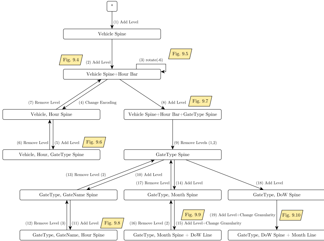
Fig. 8.18 Exploration strategy for instant time with intermediate visualisation steps and unique transformations.
