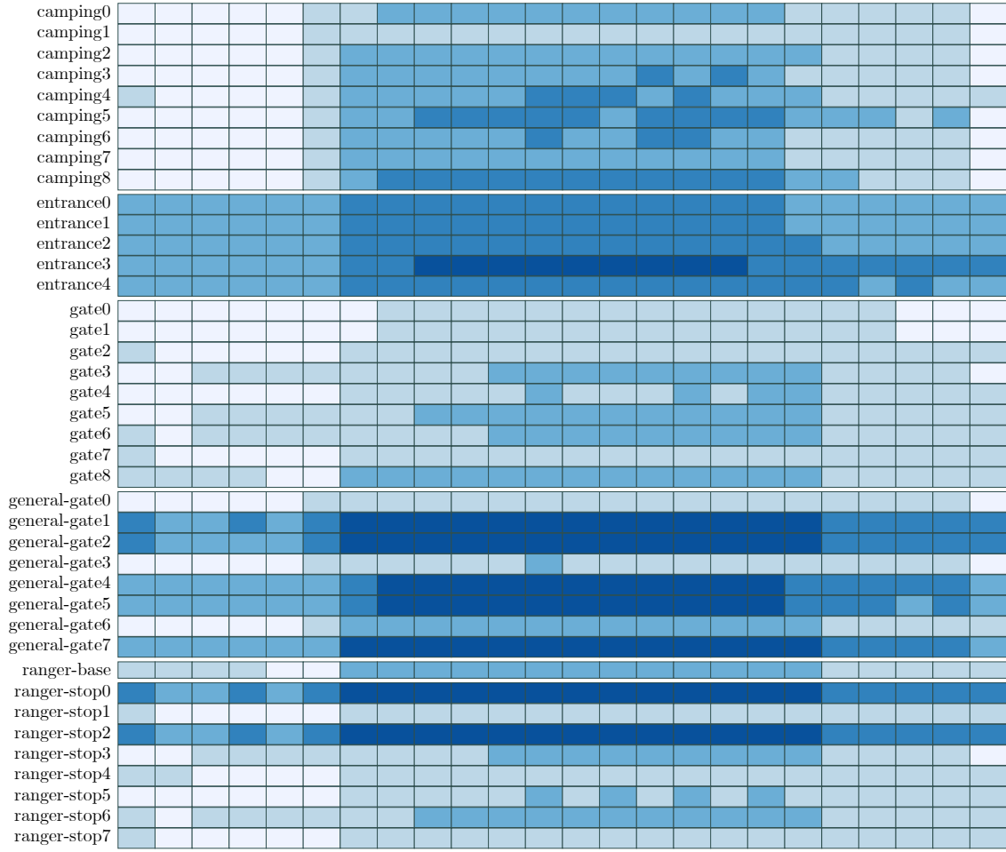
Fig. 8.8 Heatmap for GateType, GateName and Hour for specification in table 8.3. Signature: N(\text{GateType}, L_1), N((\text{GateName}, L_2), (\text{Hour}, L_3))
