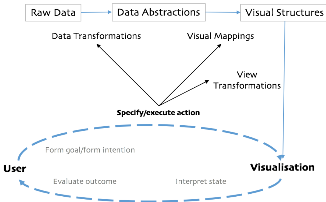
Fig. 3.3 The merged Card-Norman model. The upper part of the model describes the design phase of the visualisation, from which the major transformation steps can be reused in the execution phase, represented by the lower part of the model. The stage of specify/execute action from Norman's model is placed outside the loop and connected to the three transformation steps of Card's reference model, showing the conceptual overlap between the models.
