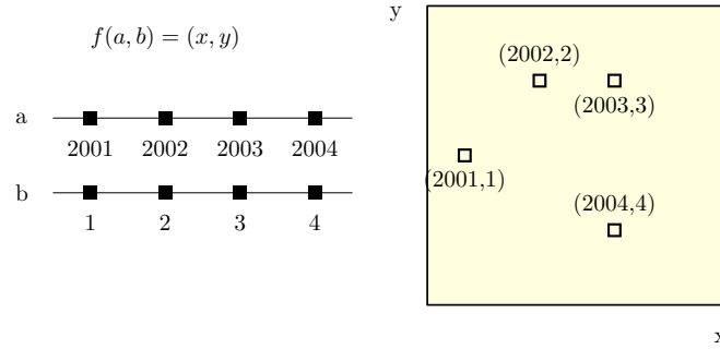
Fig. 5.4 Examples of n-to-2 layout. In the figure, function f maps two variables to the two visual dimensions x and y . This case covers layouts such as spiral formulas.
