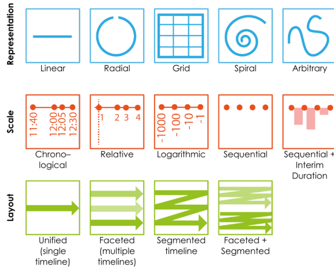
Fig. 2.4 Design space for timeline visualisation with representation, scale and layout dimensions (Brehmer et al., 2017).
