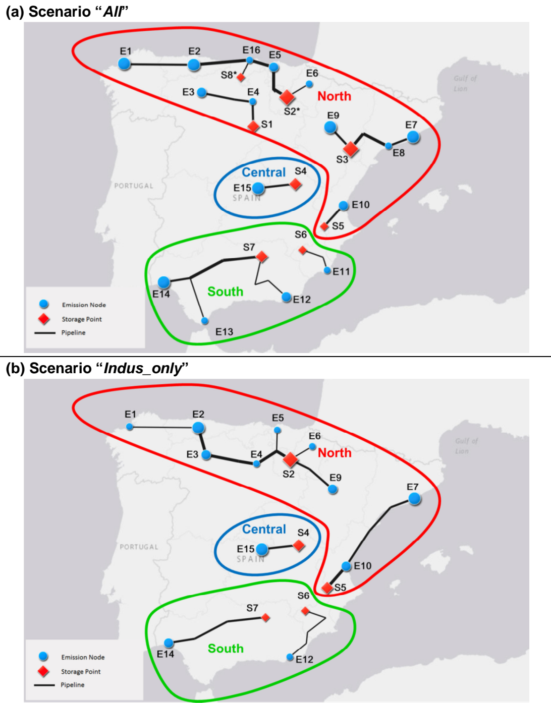
Figure 4. An illustration of the three independent subsystems
