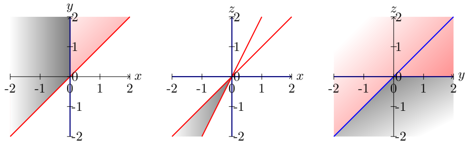
I'_0 (red) tightened to its closure I''_0 (grey)
