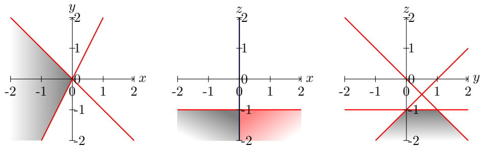
J'_0 (red) tightened to its closure J''_0 (grey)
