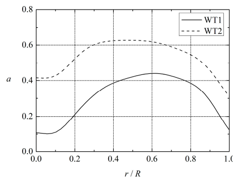
Figure 24. Radial distributions of averaged axial flow interference factors.
