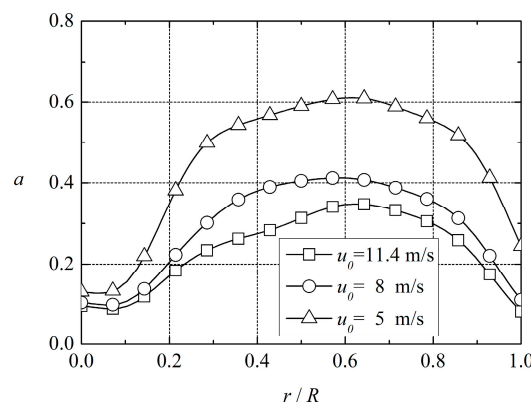
Figure 14. Radial distributions of averaged axial flow interference factors at different wind speeds.
