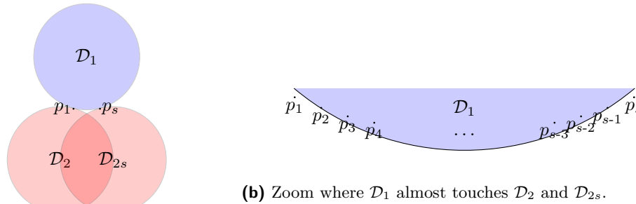
(a) Three important disks with the same size \mathcal{D}_1, \mathcal{D}_2, \mathcal{D}_{2s} .
