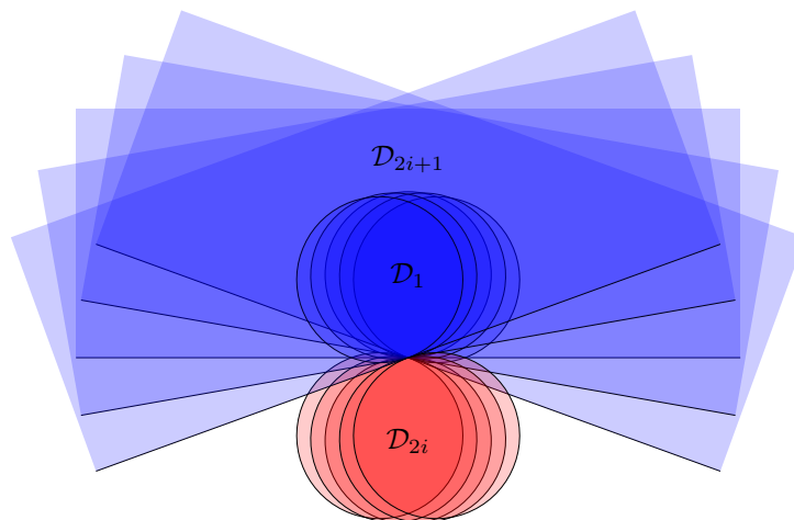
■ Figure 6 A disk realization of the complement of the disjoint union of an arbitrary number of even cycles. The rectangles symbolize the large disks; the ones with odd index except \mathcal{D}_1 .
