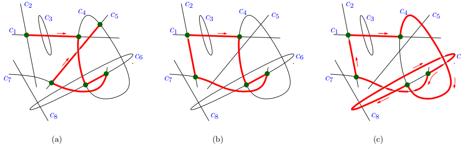
Fig. 3 Some paths in the example of Fig. 2, using the fixed intersection points marked in Fig. 2. In (a) there is a \pi -path for the walk \pi = c_2c_1c_4c_6c_7c_5c_4 . In (b) and (c) there are two different closed \pi -paths for the closed walk \pi = c_2c_1c_4c_6c_7c_2 .
