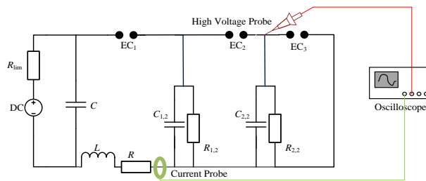
Fig. 6. Experiment system
