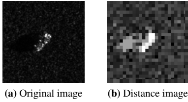
Fig. 2: Distance image between the extracted GMMs and background model
