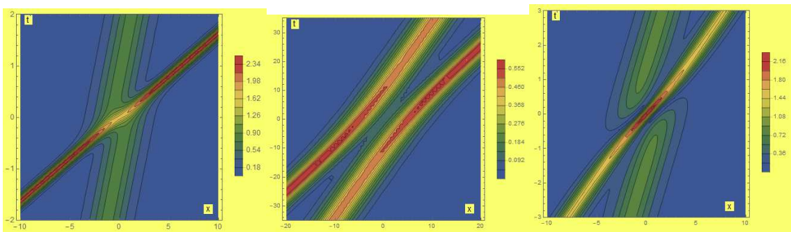
Figure 3: Different types of nondegenerate two-soliton scattering processes for the solution (3.11). Left panel: merge-split scattering with \alpha = 1.1 , \beta = 0.9 , \rho = 2.5 , \xi = 0.4 , \delta = -0.8 , \sigma = 0.6 . Middle panel: bounce-exchange scattering with \alpha = 1.1 , \beta = 0.9 , \rho = -0.6 , \xi = 0.1 , \delta = 0.5 , \sigma = 0.2 . Right panel: absorb-emit scattering with \alpha = 1.1 , \beta = 0.9 , \rho = -1.5 , \xi = 0.4 , \delta = -0.8 , \sigma = 0.6 .
