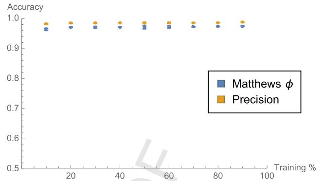
Fig. 4. The learning curve for the (enhanced) 1.54 M data for h^{1,1} \leq 12 CICY 4-folds on distinguishing elliptic fibrations.
