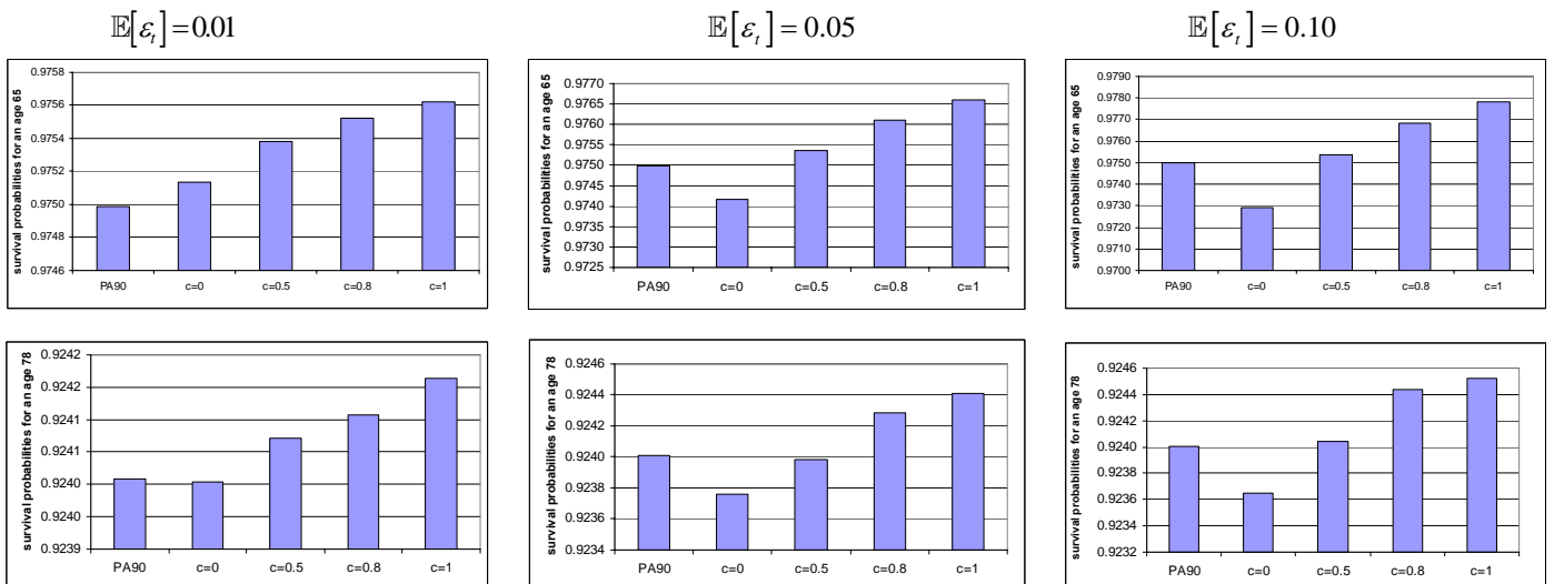
Figure 2: Comparison between CMI tables and adjusted tables by varying c and the parameters of beta distribution
