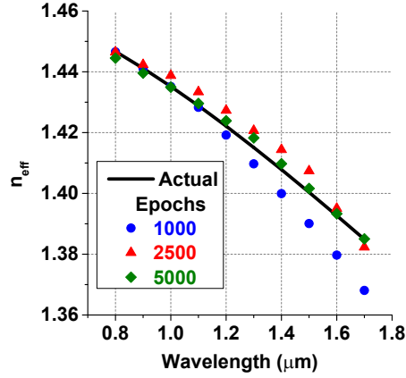
Fig. 4: Comparing actual (simulation) and predicted (ANN model) n_{eff} for different epochs at an unknown pitch, \Lambda = 1.5 \mu\text{m} , d/\Lambda = 0.7 , and N_r = 4 .
