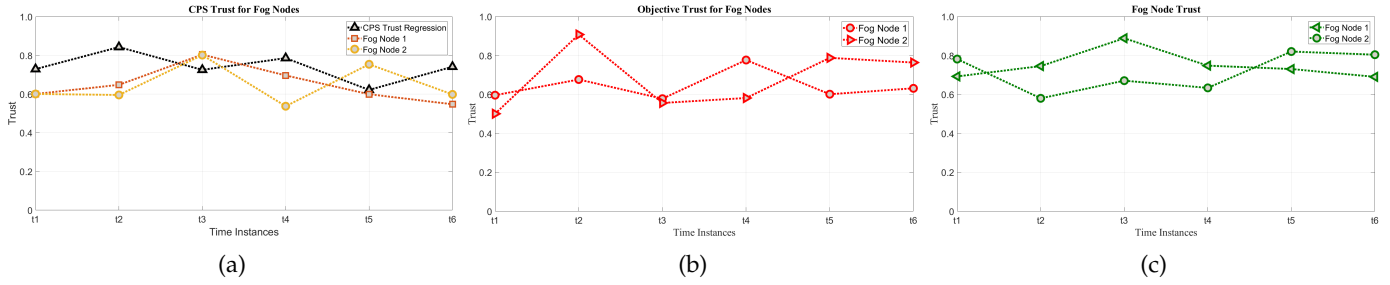
Fig. 4: Fog Nodes Trust in Hostile free Environment
