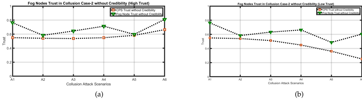
Fig. 7: Fog Nodes Trust without Credibility in Hostile Environment ( Second Case C 2 )
