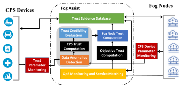
Fig. 2: Fog-CPS Trust Management System
