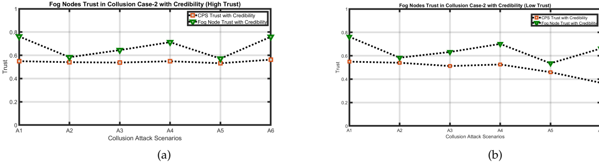
Fig. 8: Fog Nodes Trust with Credibility in Hostile Environment ( Second Case C 2 )
