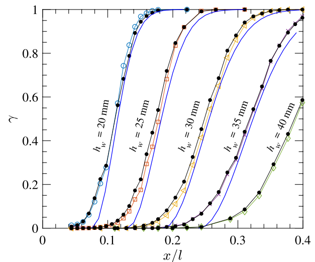
Fig. 14 Streamwise intermittency distributions for various heights ( h_w ) of the aerofoil. Symbols: hollow markers—using proposed method; solid marker—dual-slope method; solid line—Narasimha (1957)
