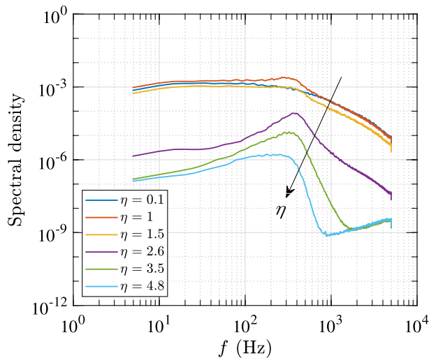
Fig. 3 Power spectral density of the aerofoil wake measured at x/c = 0.8 for various wall-normal stations; Re_c = 3.4 \times 10^5
